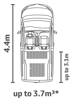
Short wheelbase panel van
